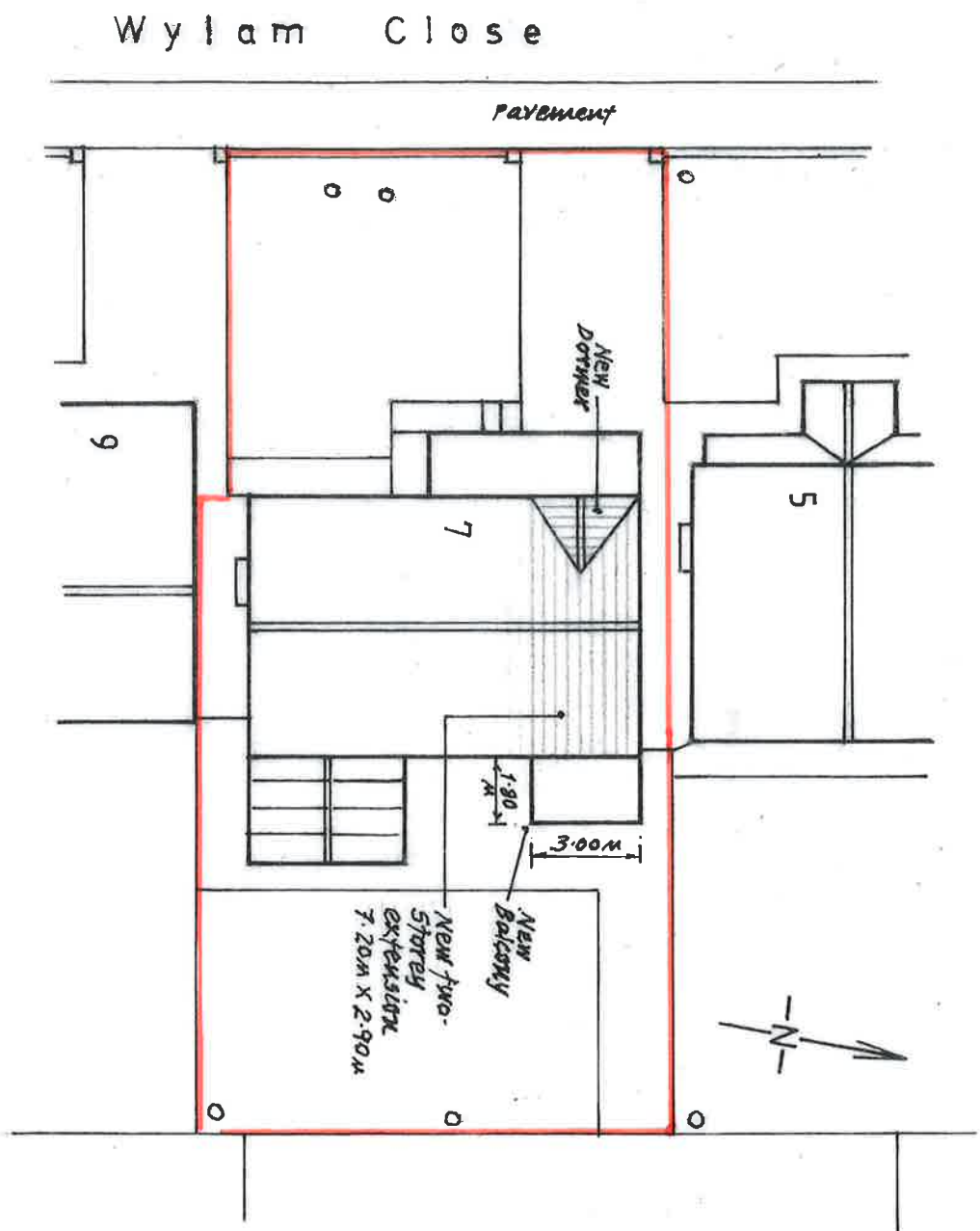
PROPOSED SITE / ROOF PLAN 1:200
